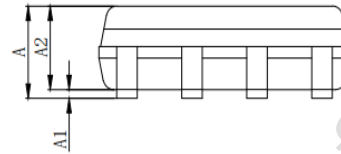
Figure 22. SOP-8 Side View
