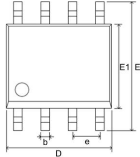
Figure 21. SOP-8 Top View
