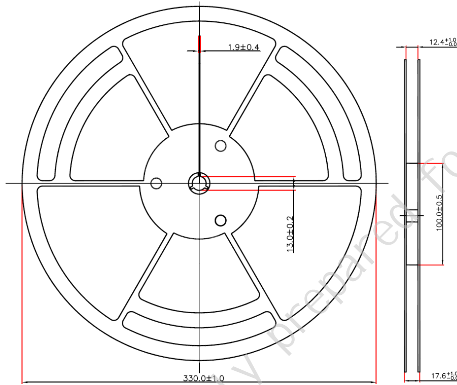
Figure 25. Reel Dimensions
