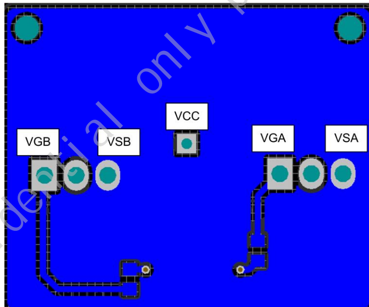
Figure 19. MK1626 Demo Board Layout (Bottom Layer)
