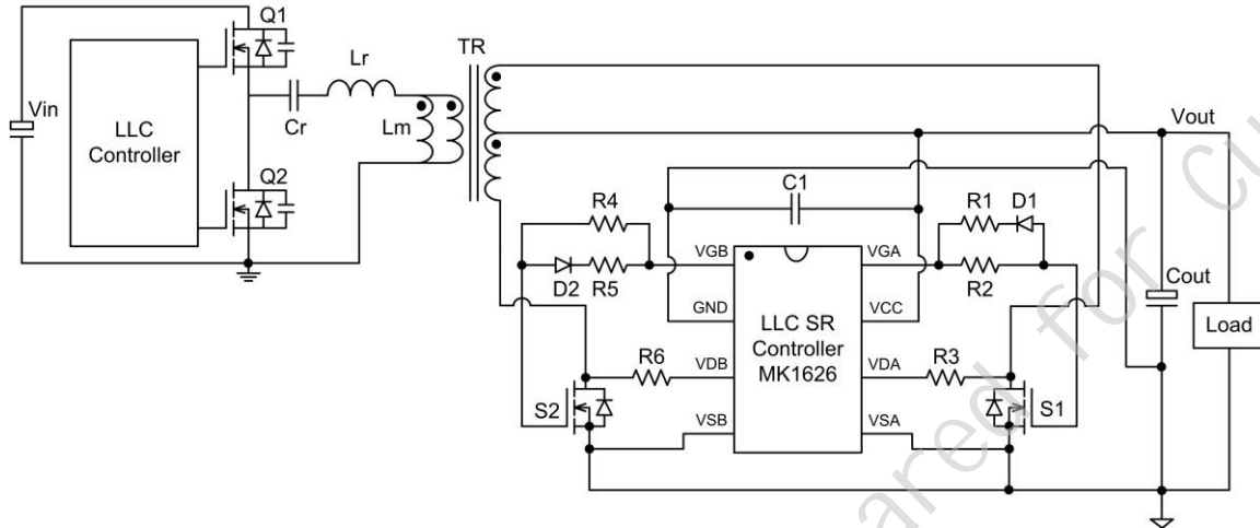
Figure 17. MK1626 Reference Design Circuit
