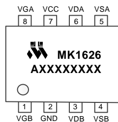
Figure 2. Pin Function (top view)
