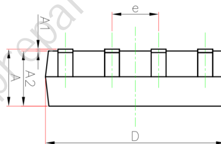
Figure20. MK9018 Side View
