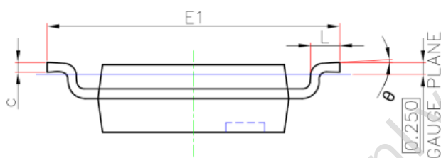
Figure19. MK9018 Side View
