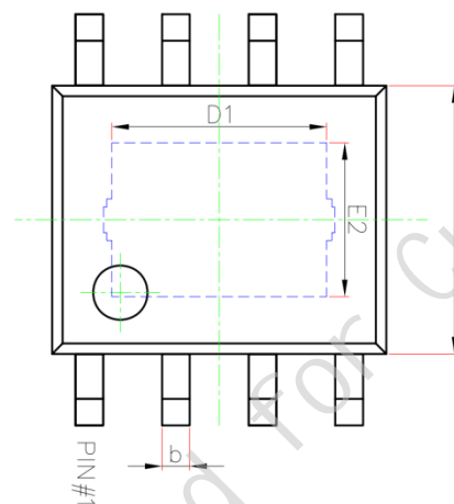
Figure 18. MK9018 Top View
