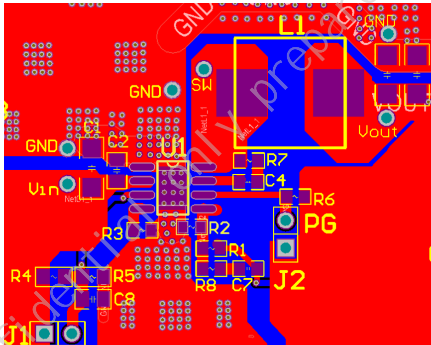
Figure16. Layout Example
