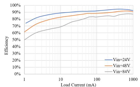
Figure 2. Efficiency at 5Vout
