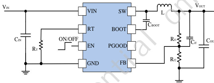
Figure 1. Typical Application Diagram
