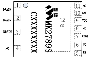
XXXXXXXX: Lot Code DFN6X8 Top View
