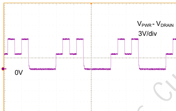
Figure 14. Detection with invalid PD (15k \Omega )
