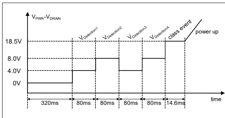
Figure 17. Type 1 Detection, Classification, and Port Power-Up Sequence
