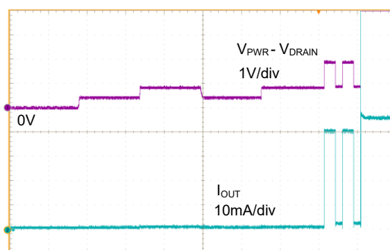
Figure 18. Classification with PD Class 4
