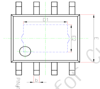
Figure 20. MK3614H Top View
