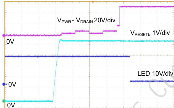
Figure 20. LED function of the PD powered from V_{RESETb}
