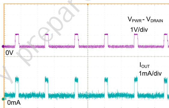
Figure 16. Detection with output shorted
