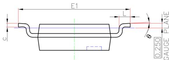
Figure 21. MK3614H Side View
