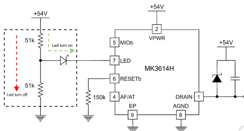
Figure 26. Recommended LED connection circuit
