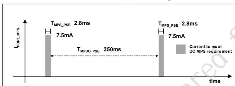
Figure 25. The MK3614H MPS requirements
