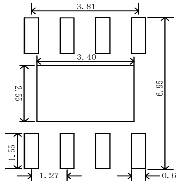
Figure 19. Recommended Land Pattern (mm)
