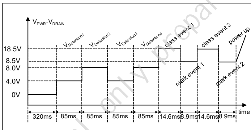
Figure 18. Type 2 Detection, Classification, and Port Power-Up Sequence
