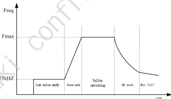
Figure 2: operation curve
