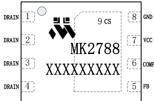
XXXXXXXXXX: Lot Code DFN5X6 Top View
